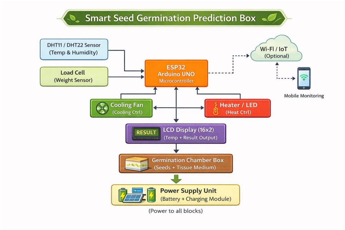
Fig.1 Block diagram of smart seed germination prediction box.
