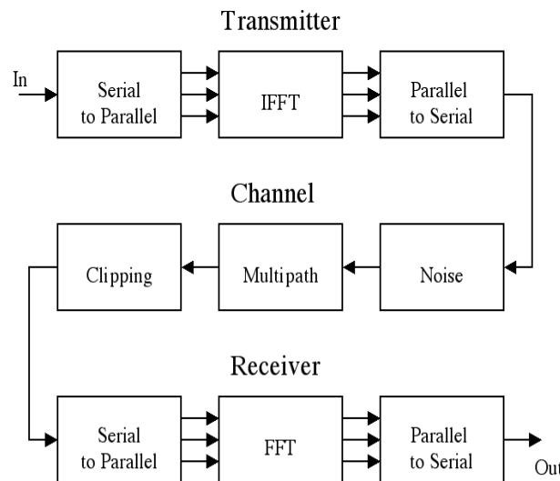
Figure 2 . OFDM model
