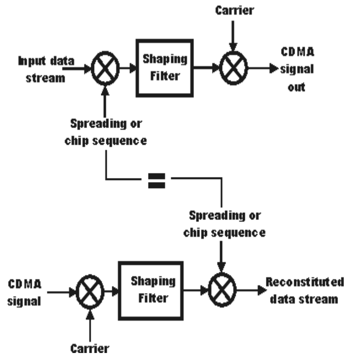
Figure 1. CDMA system showing use of spreading codes
