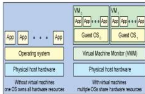
Fig. 3. Physical machine with VM and without VM
